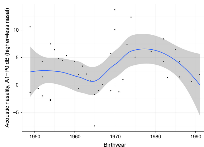
Fig. 2. Acoustic nasality ( A1-P0 ; small=more nasal) speaker means by speaker birthyear, from the trend sample, fit with a loess curve.
