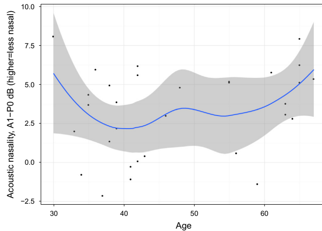
Fig. 3. Acoustic nasality (A1–P0) speaker means by speaker age, from the pseudo-panel sample, fit with a loess curve.
